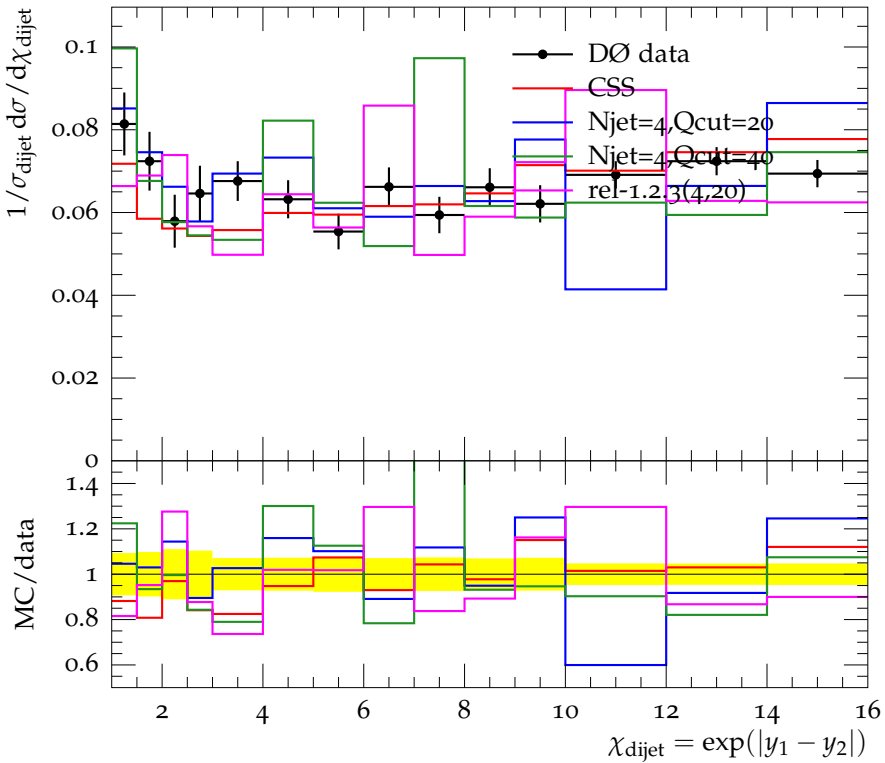
Dijet angular distribution in 0.6 < M_{jj}/\text{TeV} < 0.7
