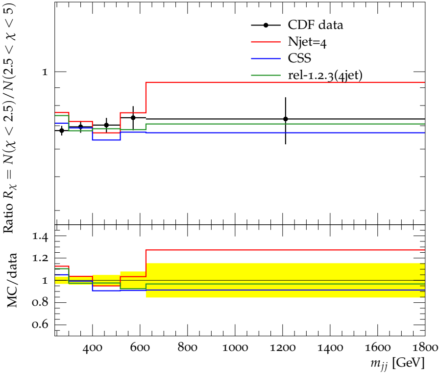
Dijet angular ratio as function of dijet mass
