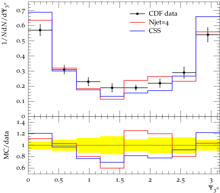
Angular distribution in inclusive 5-jet events
