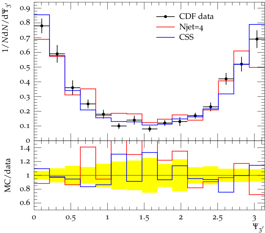
Angular distribution in inclusive 4-jet events
