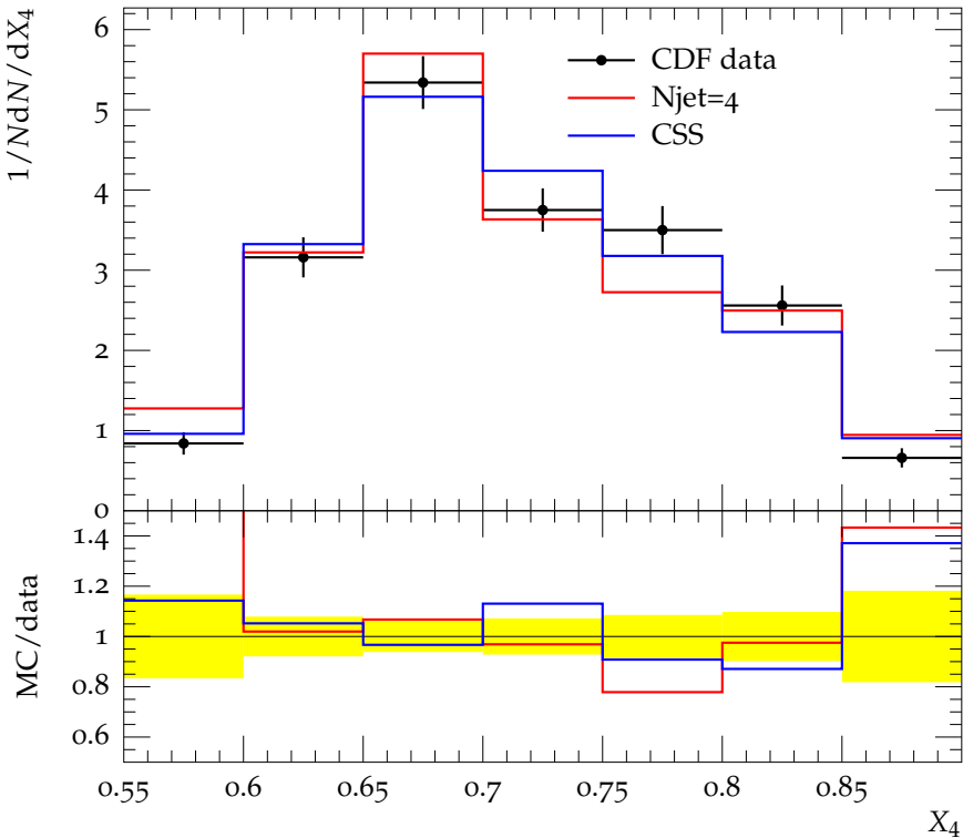
Dalitz distribution in inclusive 3-jet events
