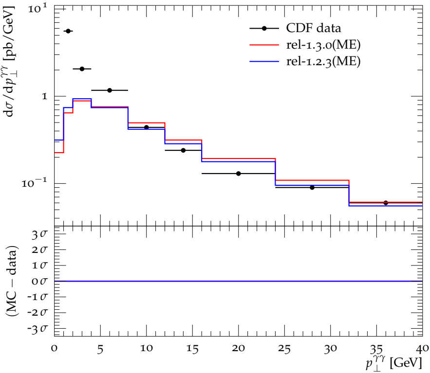
Transverse momentum of diphoton pair (compared to DIPHOX)
