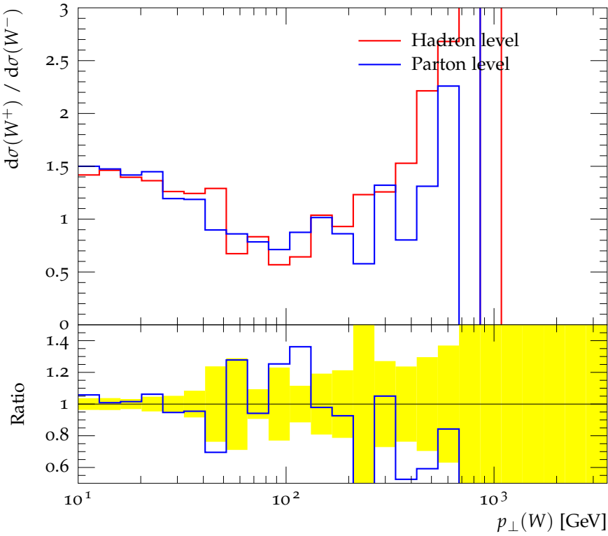
Charge asymmetry vs. p_{\perp}(W)
