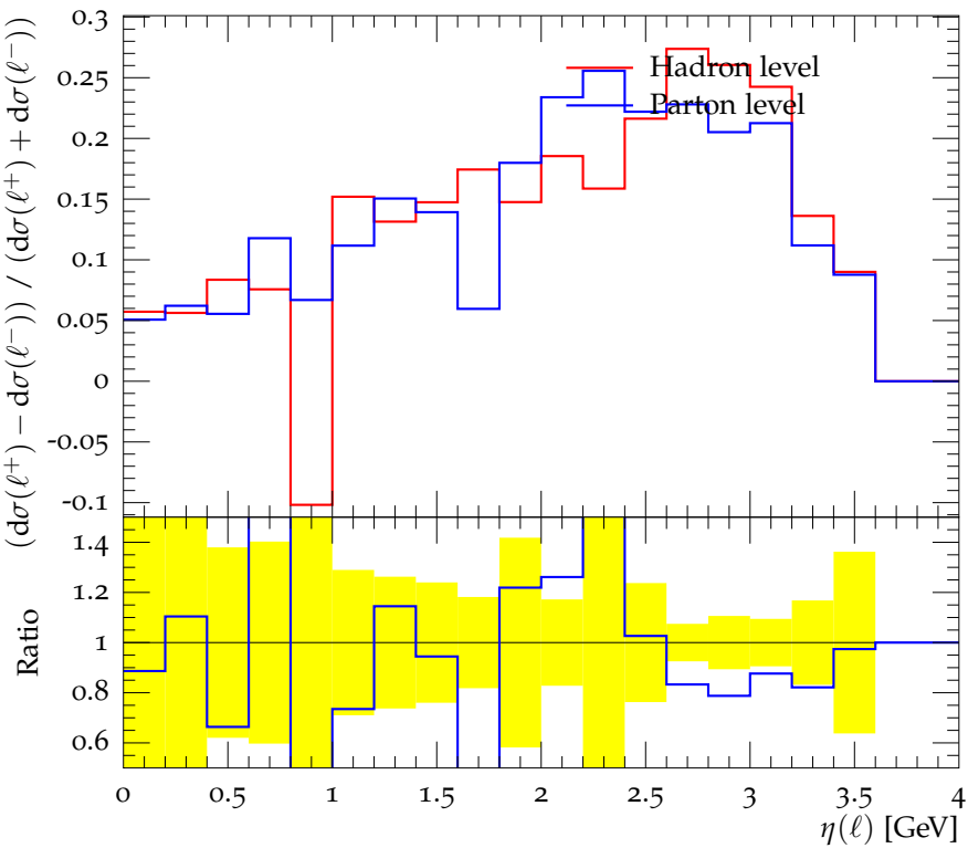
Charge asymmetry vs. \eta(\ell)
