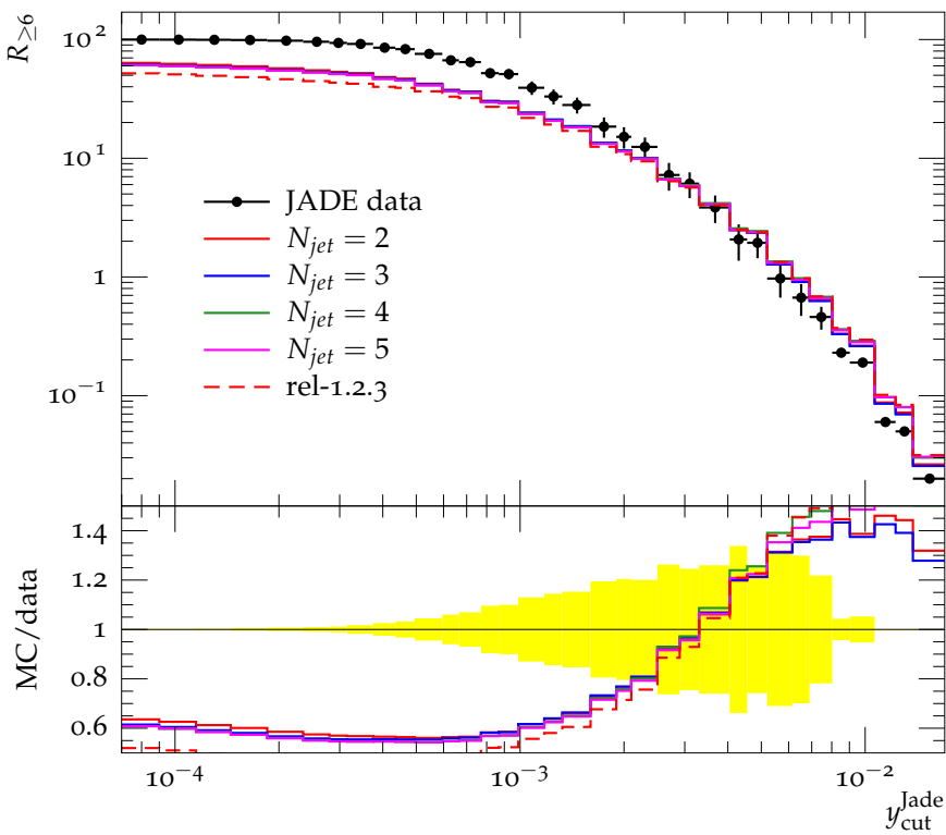
Integrated \geq 6 -jet rate with Jade algorithm (91.2 GeV)
